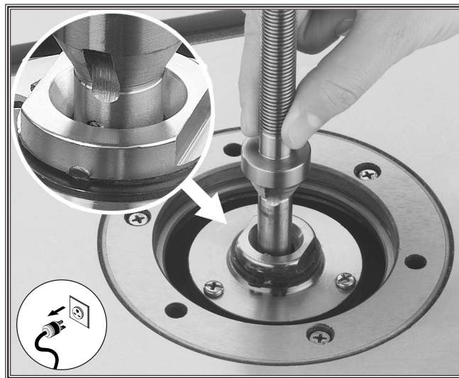
Figure 19. Spindle and guide pin alignment.
