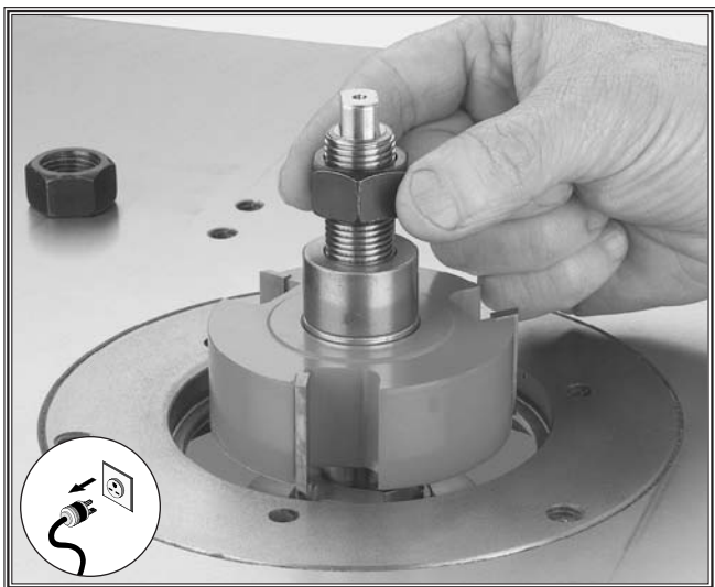
Figure 38. Spindle nut placement.
