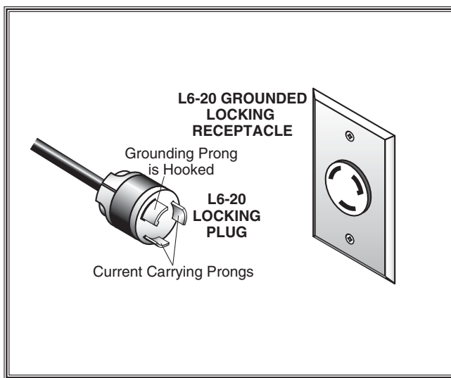
Figure 8. NEMA-style 6-20 plug and receptacle.
