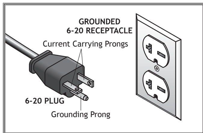
Figure 2. Typical 6-20 plug and receptacle.
